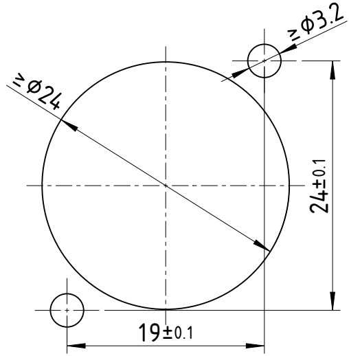
Panel cut out dimension (rear side):
