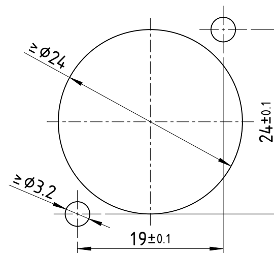
Panel cut out dimension (rear side):
