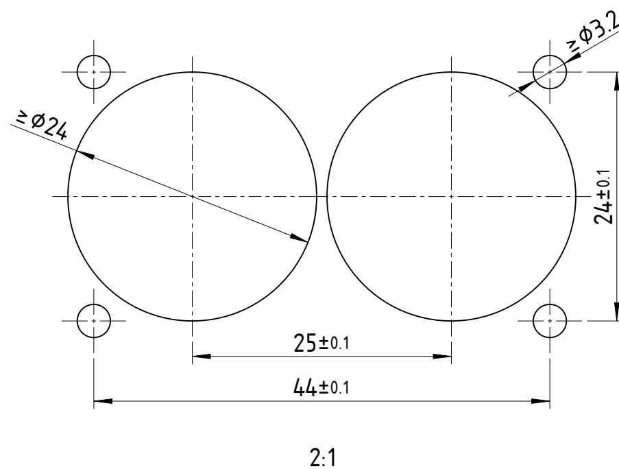
Panel cut out dimension (rear side):
