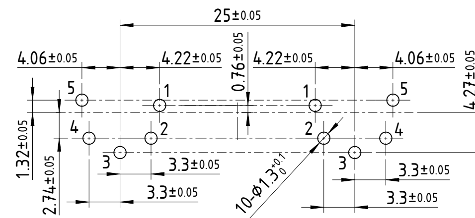
PCB cut out dimension (rear side):
