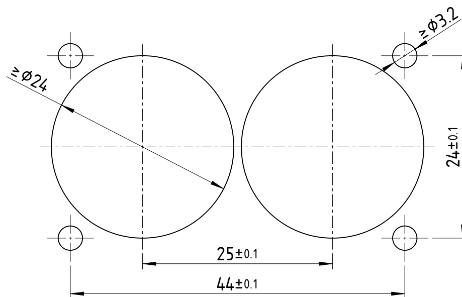
Panel cut out dimension (rear side):
