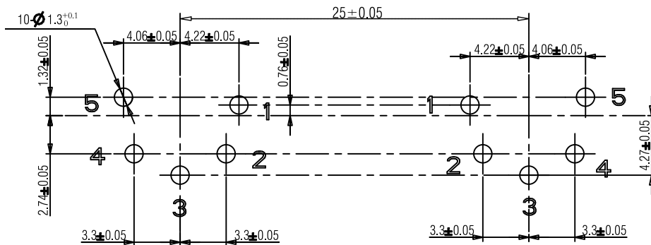
Panel Cut out dimension:
