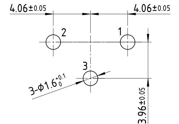
PCB cut out dimension (rear side):
