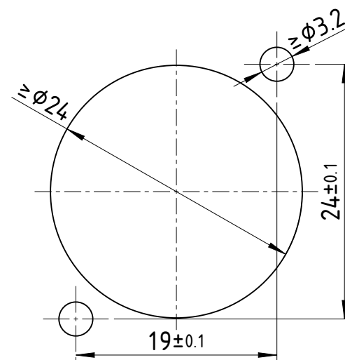
Panel Cut out dimension (rear side):
