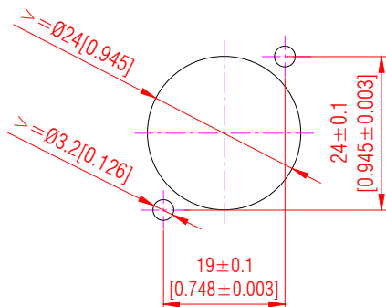
Panel cut out (Rear side)
