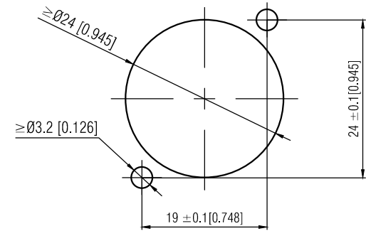
Panel Cut out dimension
