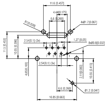
PCB Layout (Scale 2:1)
