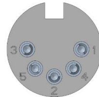
NYS322(5 Pole)
