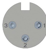
NYS321(3 Pole)
