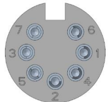
NYS323(7 Pole)
